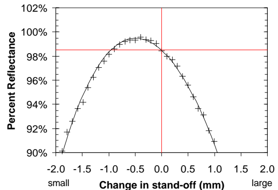
Figure 12: Effect of measurement head stand-off on color measurement. Sample measured is a white reference target. Reflectance data is averaged over the 380-780 nm range.
