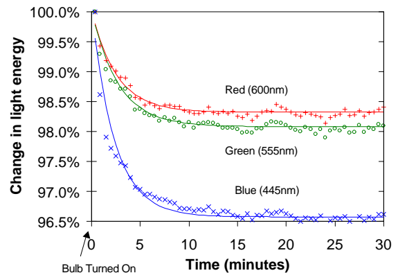
Figure 8: Effect of warm up time on light energy. Vertical axis is (\text{CCD value})/(\text{CCD value at time } 0)
